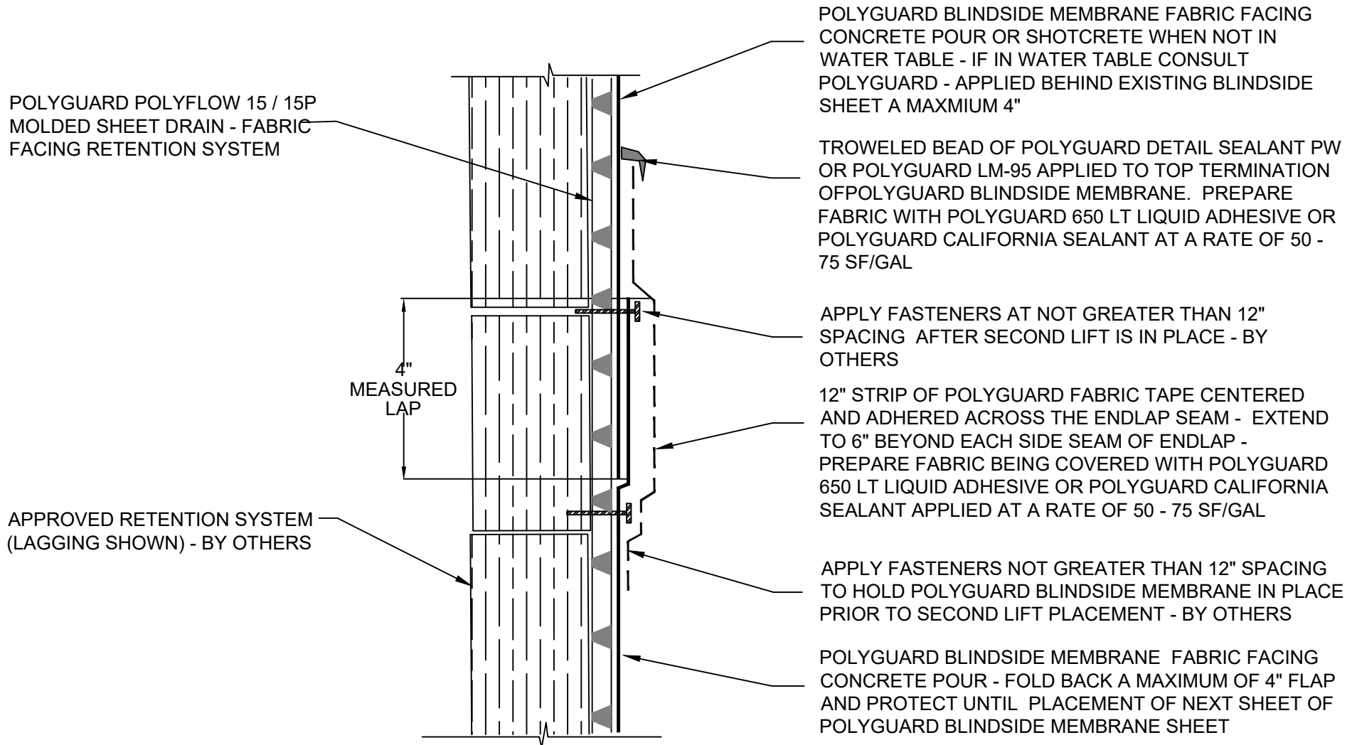
BS7 SECTION @ END LAP
