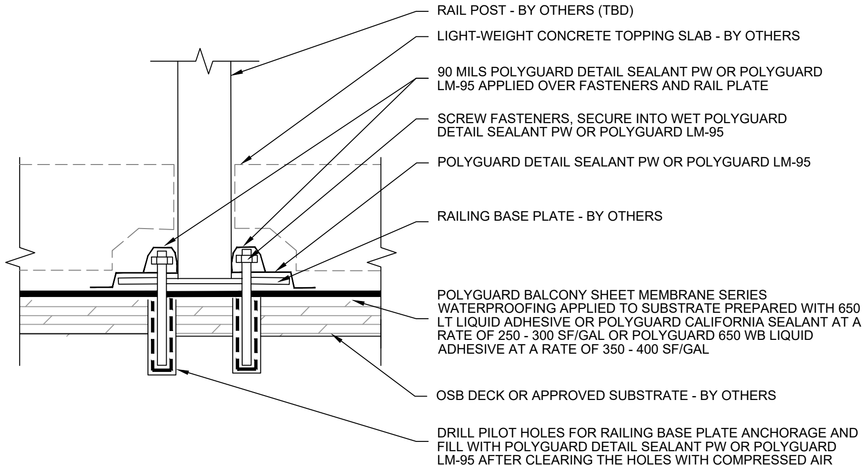
BW10 SECTION @ GUARDRAIL DETAIL (OPTION 1)
