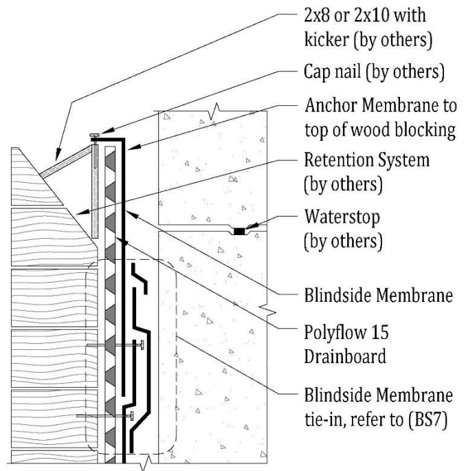
Section @ Blindside Membrane Top of Wall Termination
