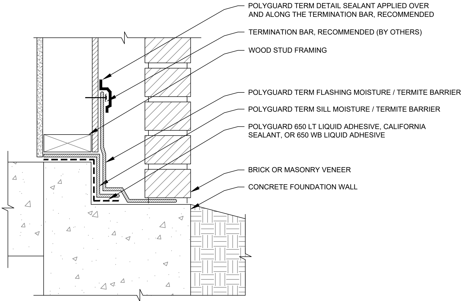
SECTION @ TERM © FLASHING / MOISTURE TERMITE BARRIER IN CAVITY WALL (FOR USE WHEN TERM © SILL / MOISTURE TERMITE BARRIER HAS BEEN PREVIOUSLY INSTALLED)
