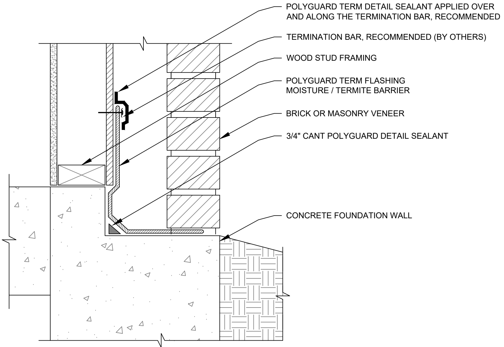
SECTION @ TERM © FLASHING / MOISTURE TERMITE BARRIER IN CAVITY WALL (FOR USE WHEN TERM © SILL / MOISTURE TERMITE BARRIER HAS NOT BEEN PREVIOUSLY INSTALLED)
